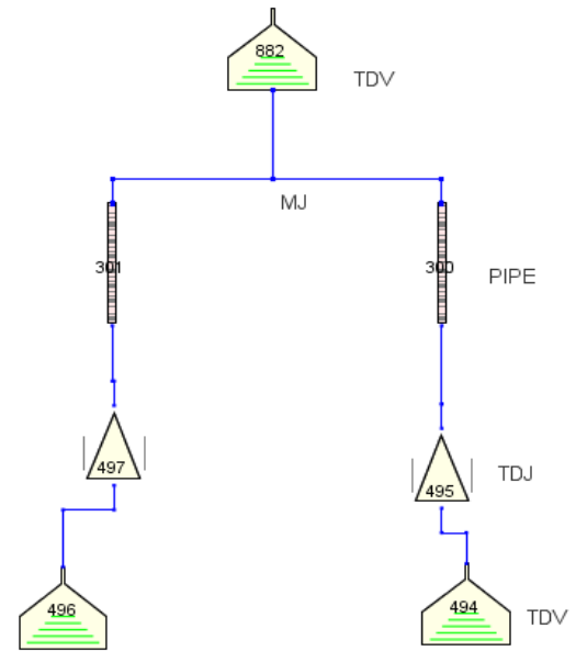
Figure 9. RELAP5-3D Nodalization.
