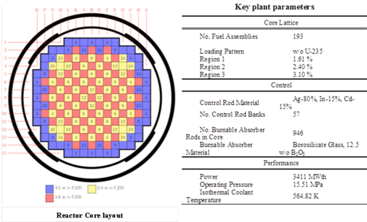
Figure 8. BEAVRS Benchmark. [40]
